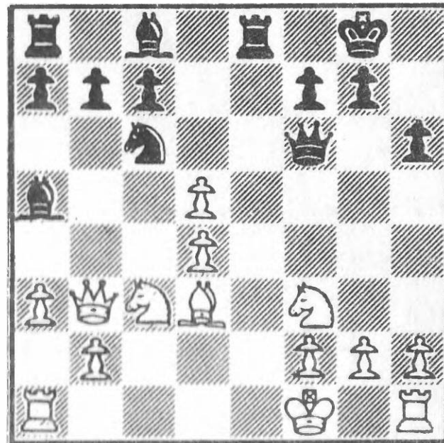
235 After 13 Kf1
